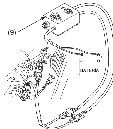
(9) Selector "PUMP"
